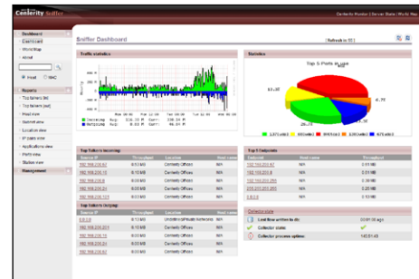
Sniffer Dashboard
